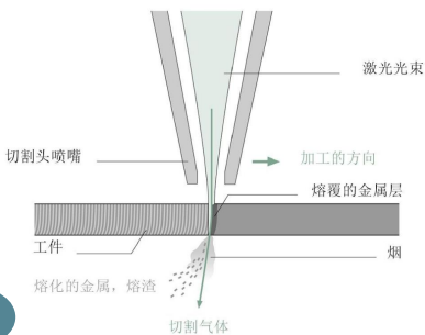
激光精确切割下料 LASER CUTTING
