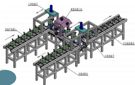
图纸的设计与验证 DESIGN AND TESTING
